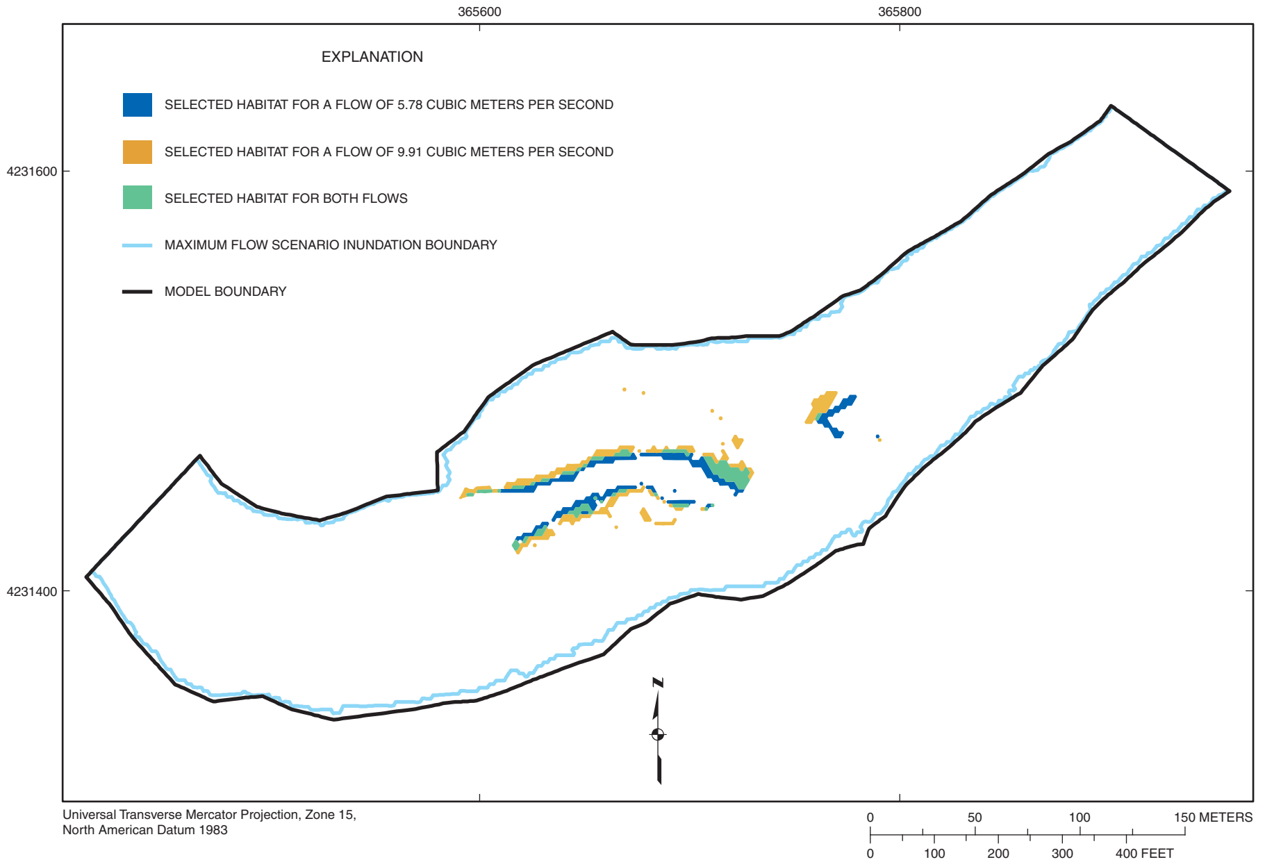
Figure 4-80. Selected habitat area distribution for habitat category 20 (flathead catfish) at flows of 5.78 and 9.91 cubic meters per second at Marais des Cygnes River site MDC2.
